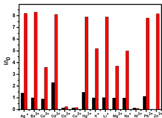
Figure 3. Fluorescence response of 1 ( 1 \mu\text{M} ) in \text{CH}_3\text{CN}/\text{CH}_2\text{Cl}_2 (1000:1, v/v) to 10 \mu\text{M} of various tested metal ions (black bar) and to the mixture of 10 \mu\text{M} of tested metal ions with 10 \mu\text{M} \text{Zn}^{2+} ion (red bar). I_0 is the fluorescence intensity for free 1 , and I is the fluorescence intensity after addition of metal ions with an excitation at 340 \text{ nm} .
