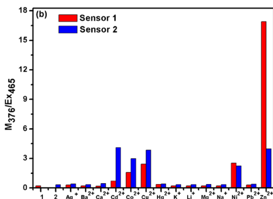
Figure 2. (a) Fluorescence spectra of compound 1 ( 1 \mu\text{M} , \lambda_{\text{ex}} = 340 \text{ nm} ); (b) ratiometric ( M_{376}/E_{465} ) selectivity of compound 1 (red bar) and 2 (blue bar) ( 1 \mu\text{M} ) upon addition of various metal ions ( 10 \text{ equiv} ) as their aqueous solutions.
