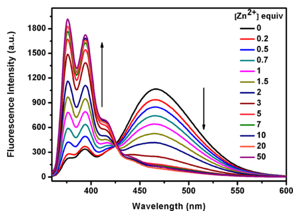
Figure 4. (a) Fluorescence spectra of compound 1 ( 1 \mu\text{M} ), upon addition of an increasing concentration of \text{Zn}^{2+} ions (0–50 equiv) measured in \text{CH}_3\text{CN}/\text{CH}_2\text{Cl}_2 (1000:1, v/v). \lambda_{\text{ex}} = 340 \text{ nm} .
